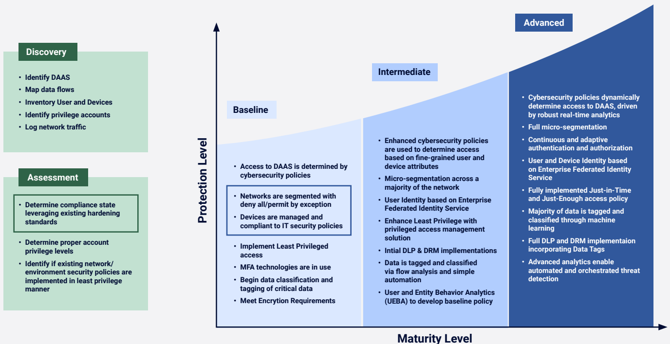
Source: Department of Defense (DOD), Zero Trust Reference Architecture, Version 1.0, February 2021
